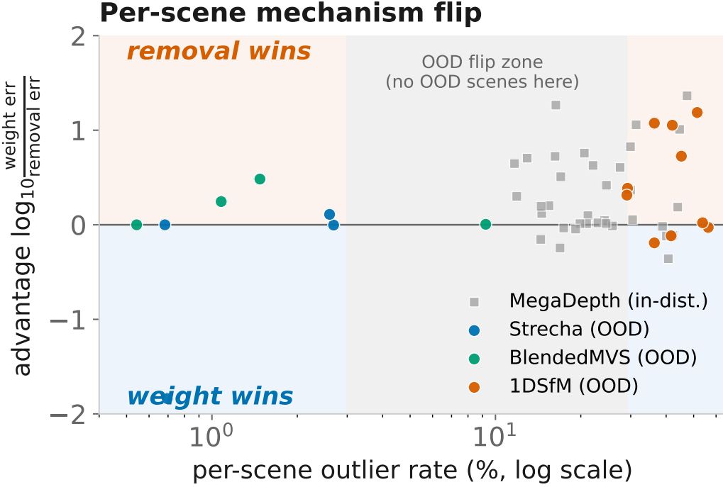
Figure 6: Per-scene complementarity (RESfM-aligned schedule). Each point is one scene: outlier rate (x, log) vs. signed advantage of removal over soft weighting. Weight wins at low contamination, removal at high contamination.
